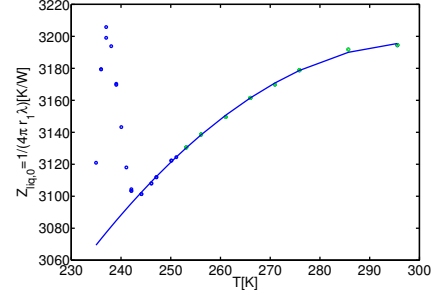
Figure 7.8 Fitted parameter Z_{liq,0} = 1/(4\pi\lambda r_1)
