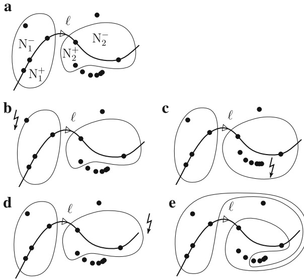
Fig. 2 Top Admissible test domain triple (N, N^+, N^-) . Middle and bottom Non-admissible test domain triples. Middle left \sigma(A) \cap \partial N \neq \emptyset . Middle right \dim P_N(A) = +\infty . Bottom left \overline{N^0} = \overline{N} \cap \ell not satisfied. Bottom right N \cap \ell not connected while N connected
