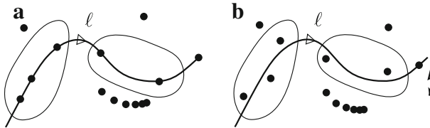
Fig. 4 A curve of closed linear relations with admissible spectra may fail to become spectral-continuous near \ell due to a spectral point \lambda_0 \in \bar{\ell} \setminus \ell for s_0 (left), which moves inward on \ell for s = s_0 \pm \varepsilon (right)
