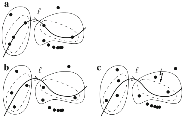
Fig. 3 Neighborhoods of the spectra of a spectral-continuous family near \ell at s_0 : The same test domain triple (N, N^+, N^-) (solid line) works at s_0 in the upper figure, at s_0 - \varepsilon in bottom left, and at s_0 + \varepsilon in bottom right. The sub-triple (N', N'^+, N'^-) (encircled by the broken line) will also work at s_0 and for s_0 - \varepsilon , but only for s_0 + \varepsilon' with \varepsilon' \ll \varepsilon
