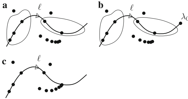
Fig. 1 Upper left closed linear relation with admissible spectrum with respect to \ell . Upper right admissible spectrum with \lambda_0 \in \bar{\ell} \setminus \ell . Bottom non-admissible spectrum since \sigma(A) \cap N \neq \sigma(A) \cap \ell and \dim \operatorname{im} P_N(A) = +\infty , each contradicting (51) (i) and (ii)
