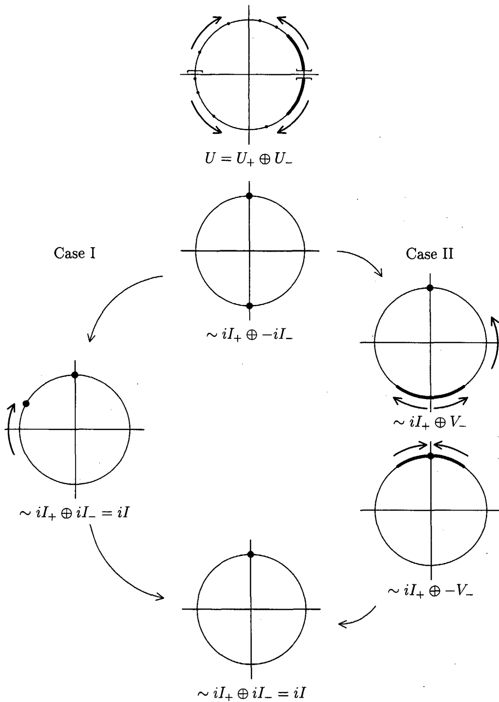
FIGURE 1. Connecting a fixed U in \mathcal{A}_{inj} to iI . Case I (finite rank U_- ) and Case II (infinite rank U_- )
